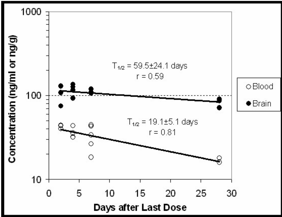
Figure 3. A semi-logarithmic plot of washout of total Hg in blood (○) and the brain (●) after 4 weekly oral doses (20 μg/kg) of methylmercury. The data were collected from groups of infants sacrificed at 2, 4, 7 and 28 days following the last dose. The lines represent nonlinear regression fit of the data to a monoexponential model. The regression estimate ( \pm standard error) of T_{1/2} is shown along with the correlation coefficient ( r ).
