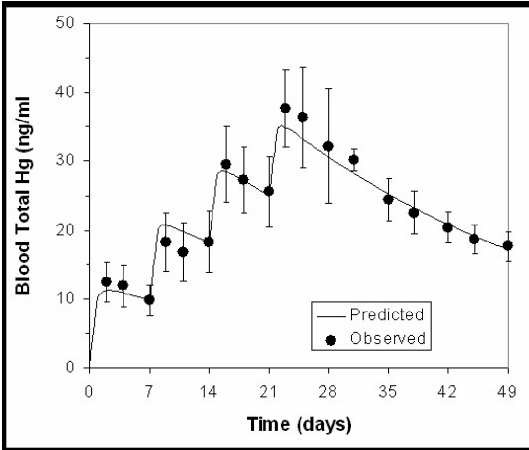
Figure 2. Comparison of model predicted and observed mean blood total Hg concentration during and after four weekly oral doses (20 \mu\text{g}/\text{kg} ) of methylmercury.
