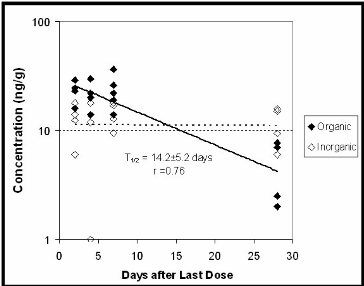
Figure 7. A semi-logarithmic plot of washout of organic ( \blacklozenge ) and inorganic ( \diamond ) Hg in the brain after 4 weekly i.m.injection of vaccines containing thiomerosal at 20 \mu\text{g}/\text{kg} of Hg. The data were collected from groups of infants sacrificed at 2, 4, 7 and 28 days following the last dose. The lines represent nonlinear regression fit of the data to a monoexponential model. The regression estimate ( \pm standard error) of T_{1/2} for organic Hg is shown along with the correlation coefficient ( r ). The half-life of inorganic Hg is too long ( >120 days) to be accurately estimated from the present data (i.e., r is not significantly different from 0).
