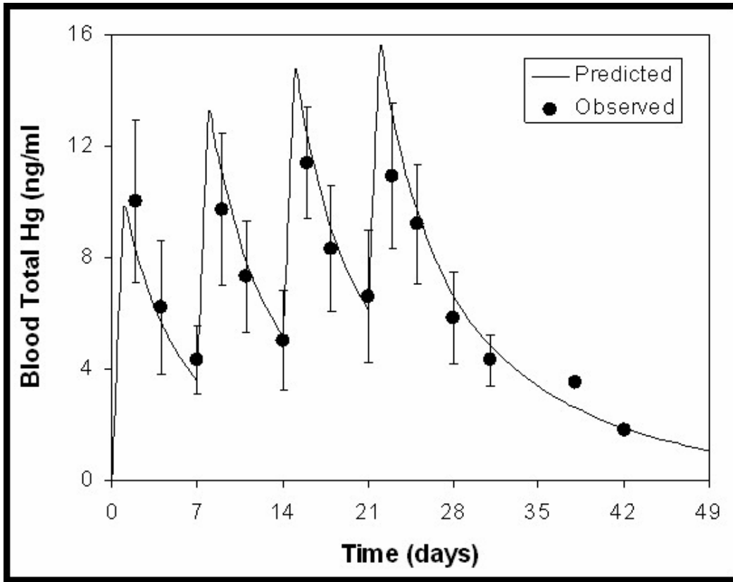
Figure 5. Comparison of model predicted and observed mean blood total Hg concentration during and after four weekly i.m. injection of vaccine containing thimerosal at 20 \mu\text{g}/\text{kg} of Hg.
